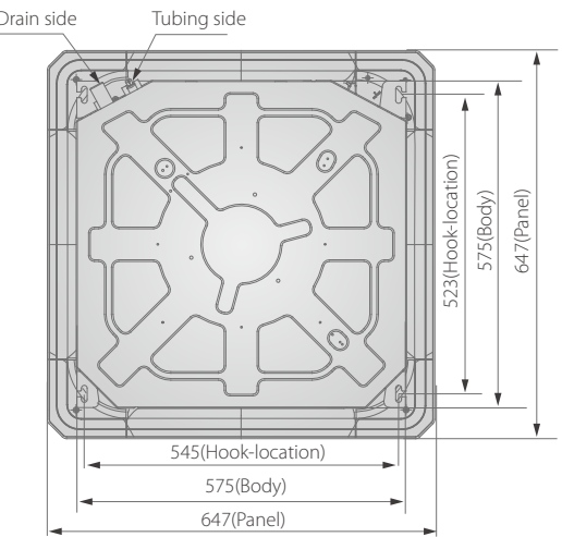
Service Spaces (unit: mm)
