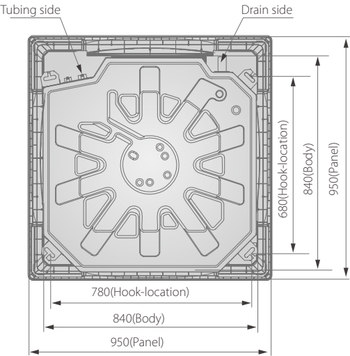
4-Pipe 4-way cassette Dimensions (unit:mm)
