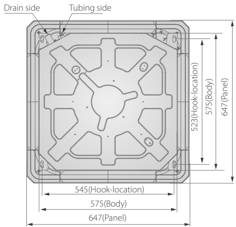
2-pipe compact 4-way cassette Dimensions (unit: mm)
