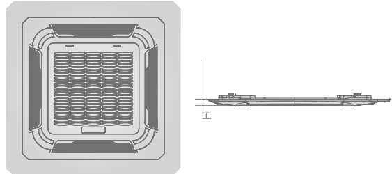
Height of the front panel
