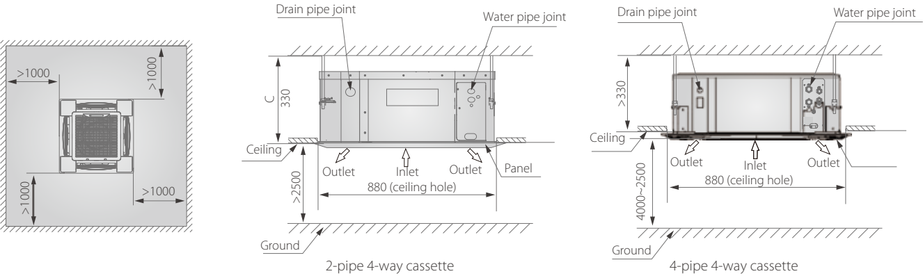
Service Spaces (unit:mm)
